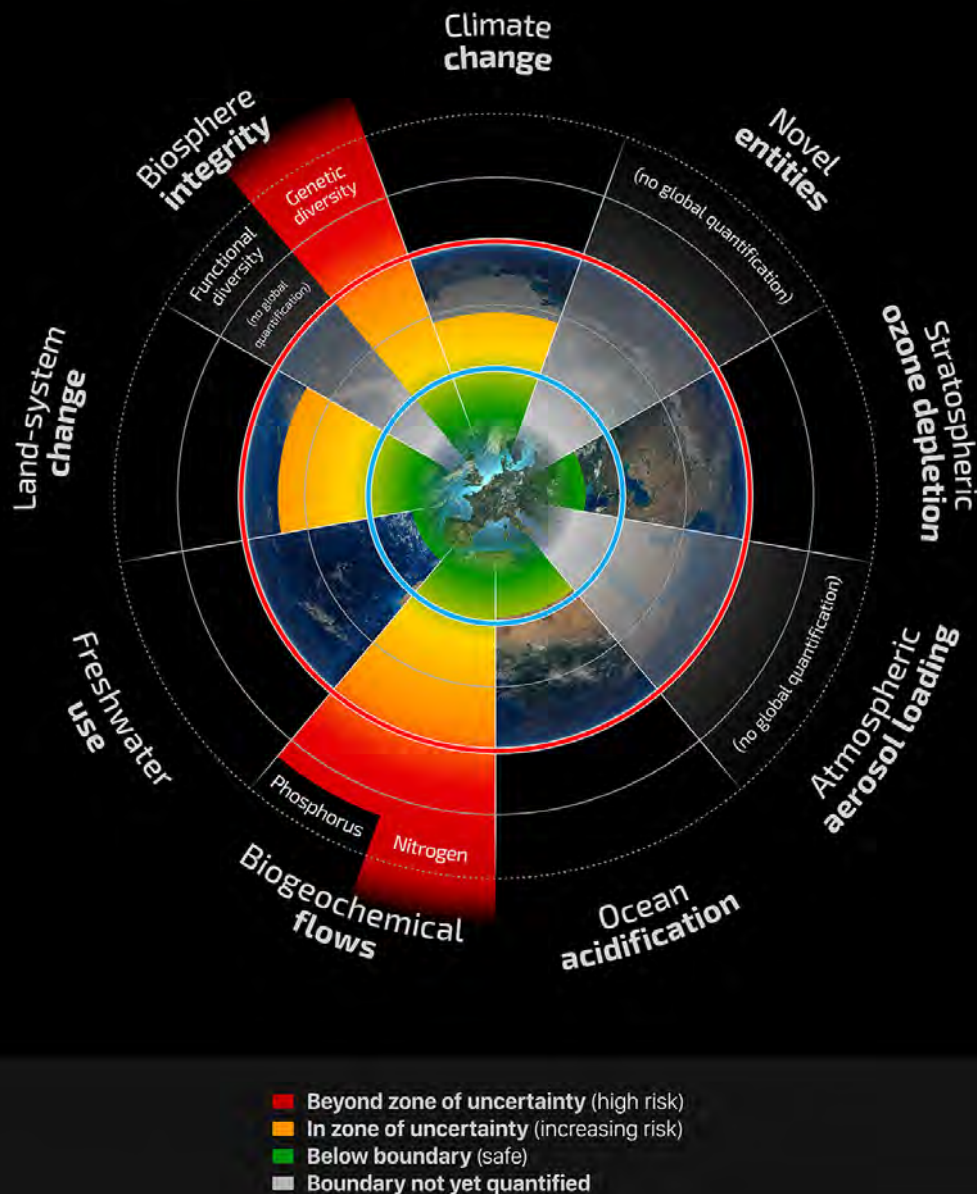
Gambar 1: Batasan-batasan Planet 7
